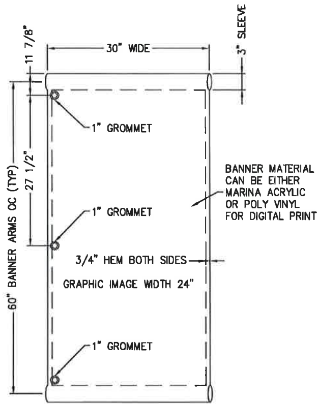
5 FOOT BANNER SCALE: NO SCALE FOR 20' TO 28' POLES
