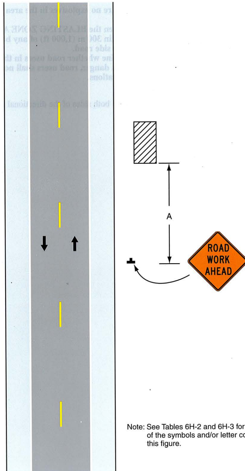
Typical Application 1
