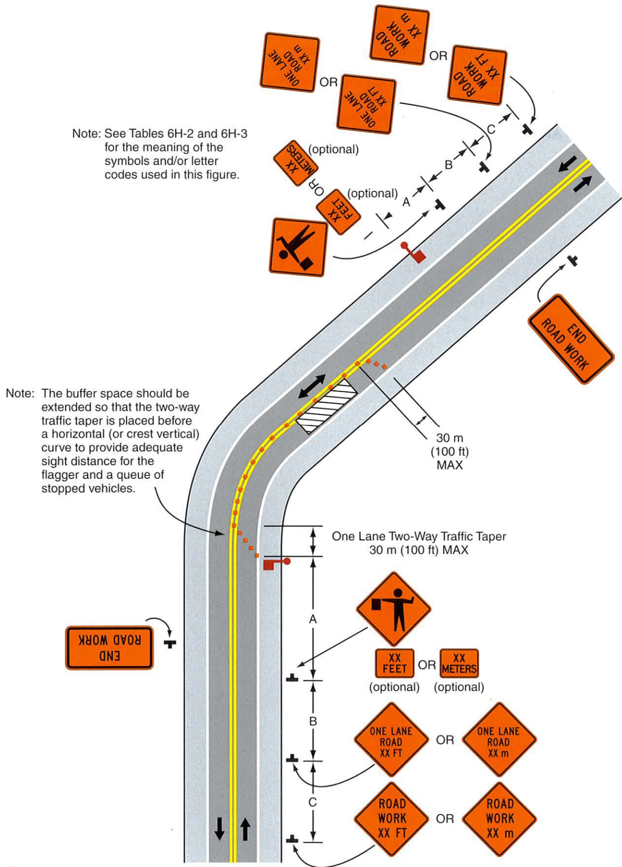
Typical Application 10
