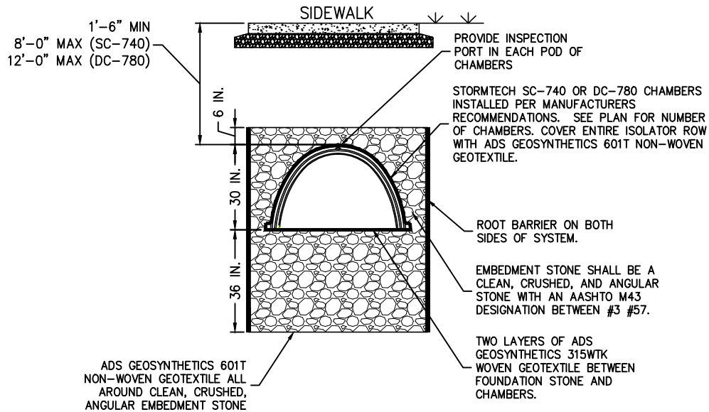
CHAMBER SYSTEM (ADS OR APPROVED EQUAL)
